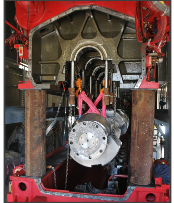
Crank Shaft Removal from Large Diesel Engine, Caribbean
